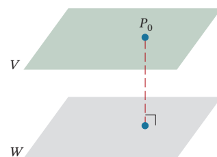
FIGURE 3.3.9 The distance between the parallel planes V and W is equal to the distance between P_0 and W .
